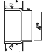
4" BOOT STANDARD CAST-IN WATERTIGHT RUBBER BOOTS AVAILABLE IN 2", 4" AND 6" SIZES
